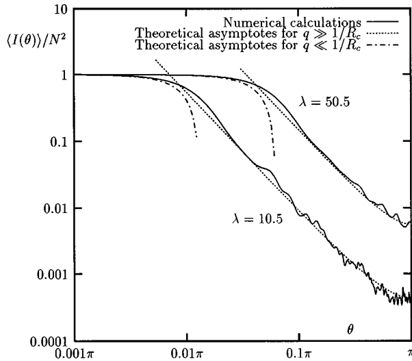
Fig. 2. Average intensity of the scattered light for \lambda = 10.5 and \lambda = 50.5 (lattice units).
