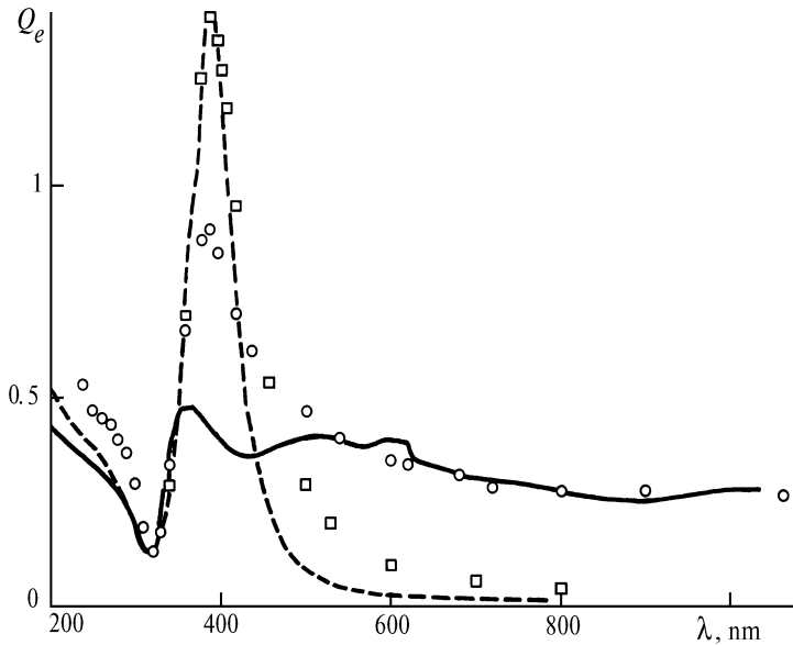
FIG. 2. Theoretical spectra of monomers (dashed curve) and clusters consisting of 30 monomers (solid curve) compared with the experimental spectra of monomers (small squares) and clusters (small circles). The fractal dimensionality of clusters is close to 1.8.
