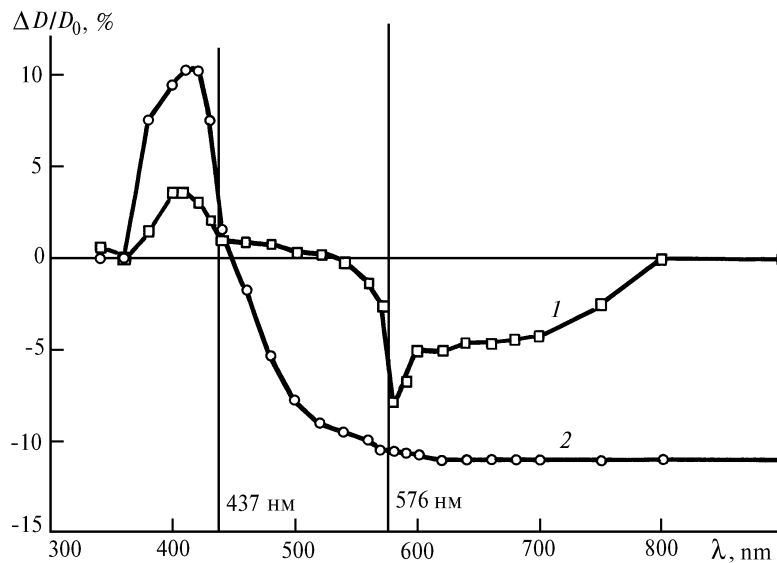
FIG. 3. Difference absorption spectra of irradiated and non-irradiated cluster samples. The cavity is 1 mm thick. The laser radiation wavelength is \lambda_1 = 576 (1) and \lambda_1 = 437 nm (2). \Delta D denotes a change in the optical density of sample, and D_0 denotes its optical density before irradiation.
