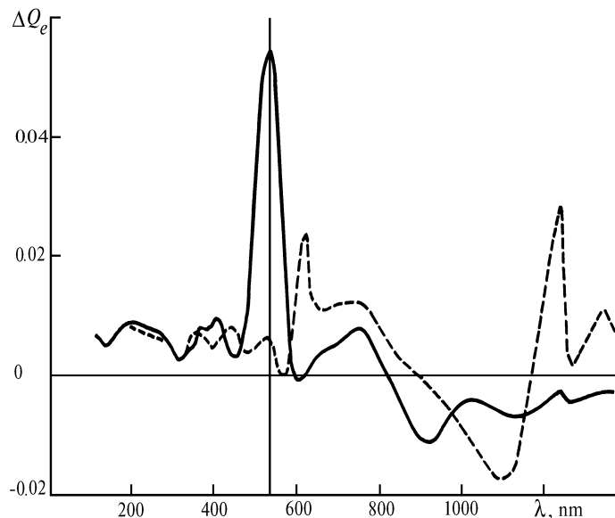
FIG. 1. Calculated difference spectra of clusters before and after irradiation by a high-power laser pulse at \lambda = 532 nm. The decrease of the absorption corresponds to the positive direction of the ordinate (spectral dip). Solid curve is for the same polarization as that of laser pulse ( \mathbf{e} \parallel \mathbf{e}_l ); and dashed curve is for the orthogonal polarization ( \mathbf{e} \perp \mathbf{e}_l ).
